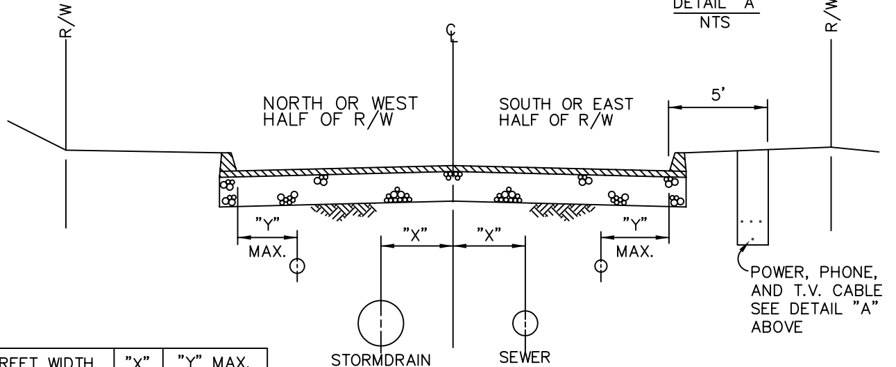
CASE II (WITH OR WITHOUT A.C. DIKE)
