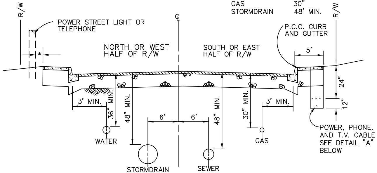
CASE I (P.C.C CURB AND GUTTER)
